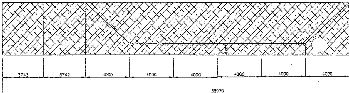
TENNIS COURT: SIDE ELEVATION SCALE 1: 100
