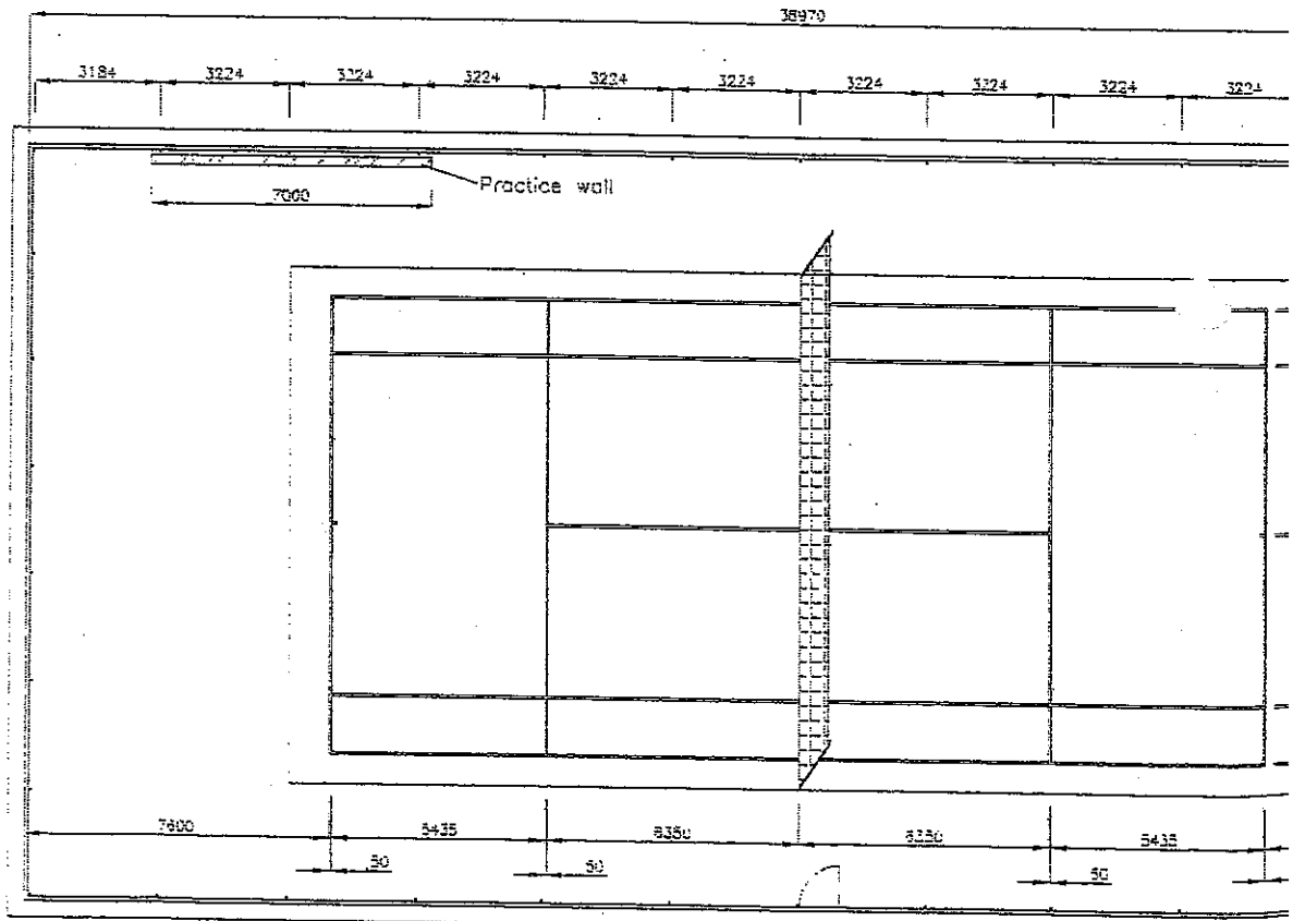
TENNIS COURT: PLAN SCALE 1: 100
