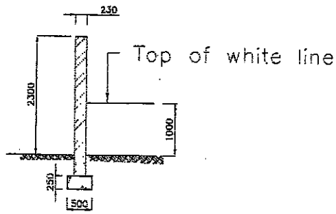
PRACTICE WALL SCALE 1: 50
