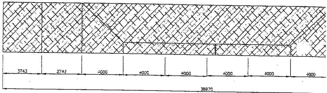
TENNIS COURT: SIDE ELEVATION SCALE 1: 100
